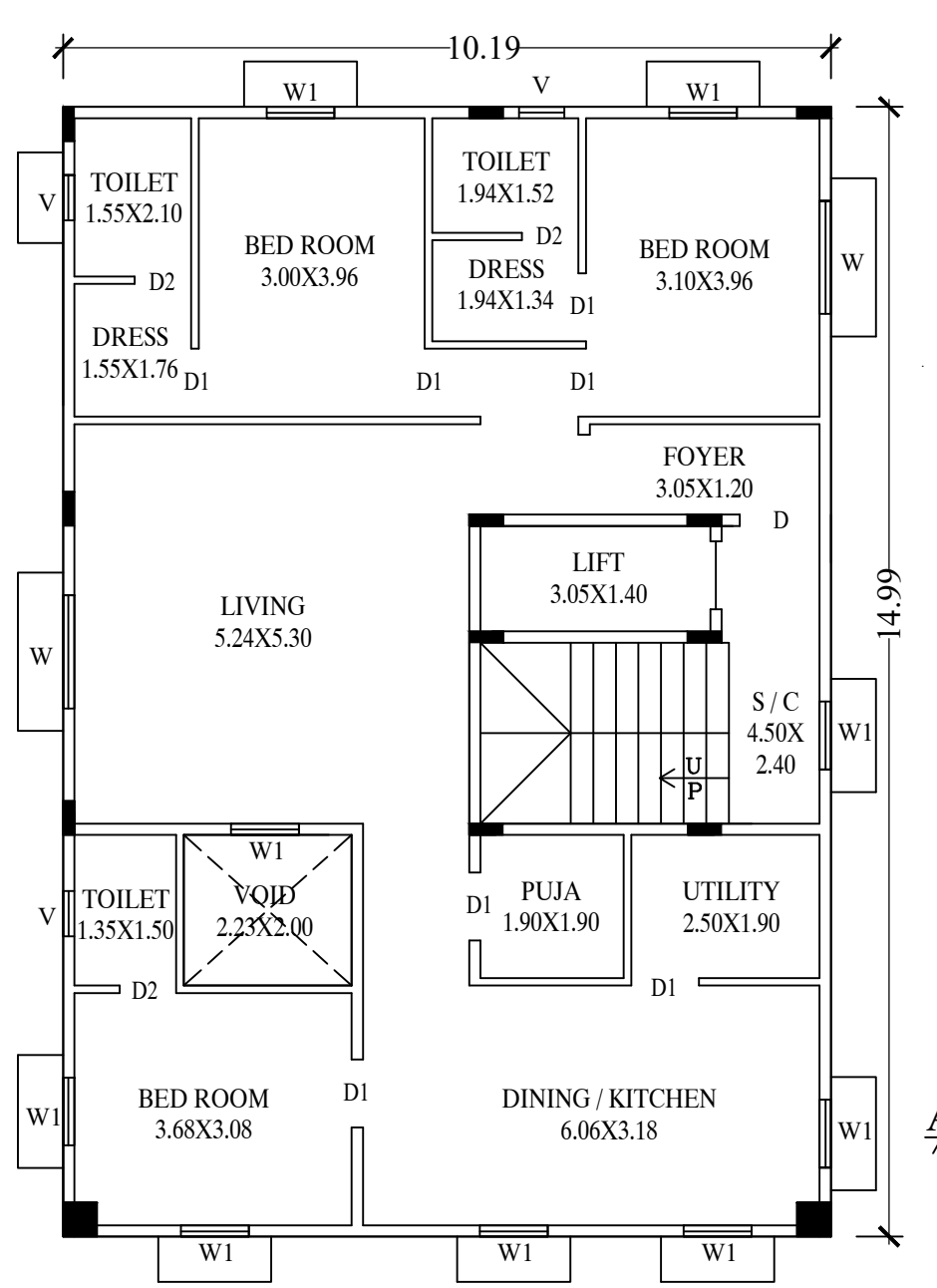
PROPOSED TYPICAL GROUND & FIRST FLOOR PLAN
